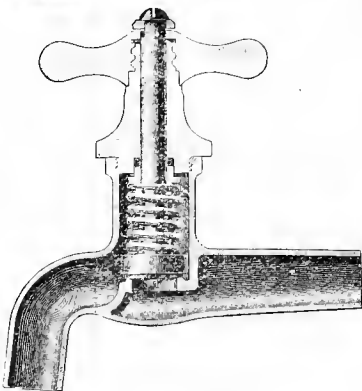
Fig. 3492. ZANE'S SELF-CLOSING BIBB-COCK.
